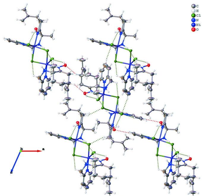
Figure 2 Intermolecular and intramolecular hydrogen bonds in the structure, shown as dashed lines.
