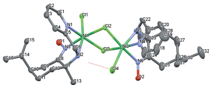
Figure 1 Displacement ellipsoid plot at the 50% probability level for Ni 2 (aminoxime) 2 Cl 4 . H atoms are omitted for clarity.
