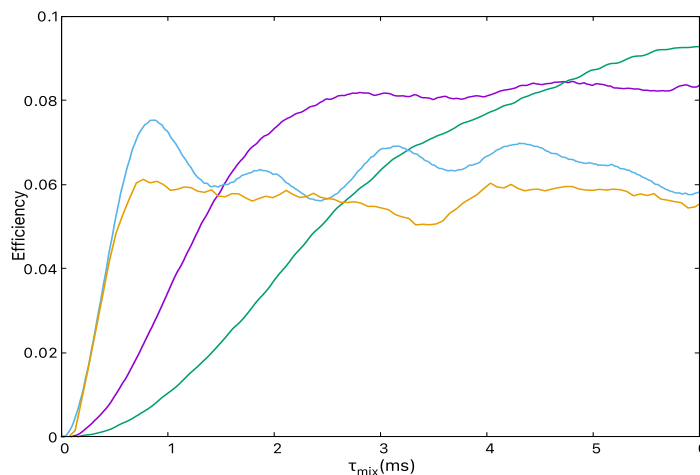
Fig.9. Simulated ^1\text{H}\{-^{14}\text{N}^{2\text{Q}}\} T-HMQC build-up curves for \{C_Q (MHz), v_R (kHz), v_1 (kHz), \alpha\} = \{3.21, 62.5, 80, 0.021\} (purple), \{3.21, 62.5, 40, 0.053\} (green), \{0.8, 62.5, 80, 0.085\} (blue) and \{3.21, 15.625, 80, 0.085\} (yellow). The \alpha parameter is calculated with Eq.26, |b_{1\text{H}-^{14}\text{N}}|/(2\pi) = 2 kHz and v_{\text{off}} = v_R .
