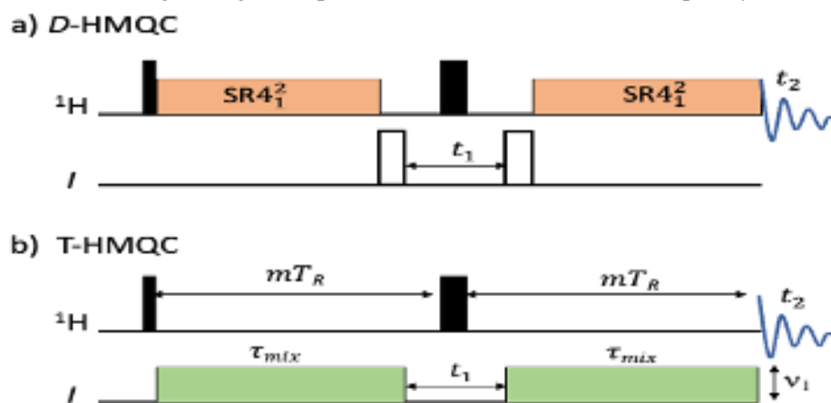
Fig.1. ^1\text{H}\{-I\} (a) D-HMQC and (b) T-HMQC pulse sequences. The ^1\text{H}\text{-}I dipolar couplings are reintroduced by applying either the \text{SR4}_1^2 recoupling on the ^1\text{H} channel with D-HMQC or two long identical pulses on the I channel with T-HMQC.
