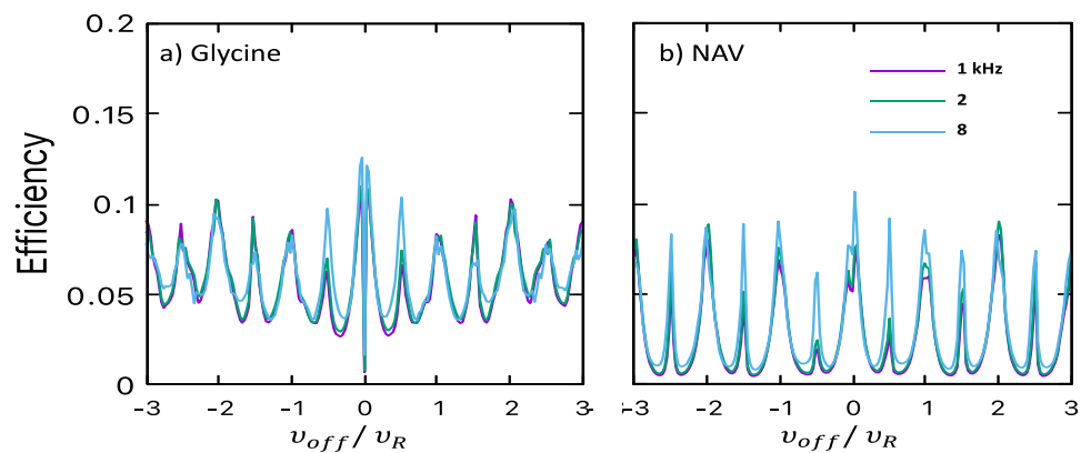
Fig.8. Simulated ^1\text{H}\{-^{14}\text{N}^{2\text{Q}}\} T-HMQC efficiency versus \nu_{\text{off}} for glycine and NAV with \nu_R = 62.5 , \nu_1 = 70 and |b_{1\text{H}-^{14}\text{N}}|/(2\pi) = 1, 2 or 8 kHz.
