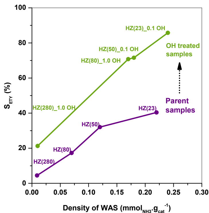
Figure 2. Correlation between the ETY selectivity (at similar ET conversion) and the density of WAS for parent (purple) and OH-treated (green) HZSM-5 catalysts tested at 225 °C, 1 bar, WHSV= 35.7 h -1 . S_{ETY} data are obtained under stable catalytic behaviors.
