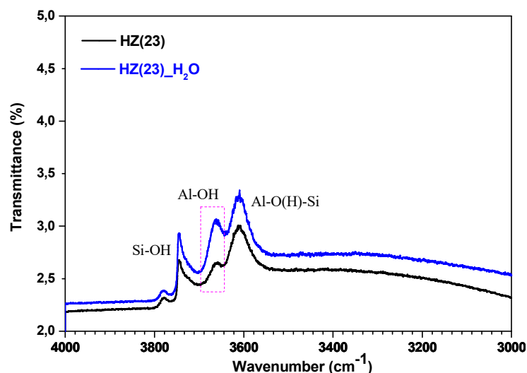
Figure 5. Normalized FTIR spectra on the OH-region for fresh parent HZ(23) and HZ(23) H 2 O samples evacuated in-situ at 350 °C (overnight) after ex-situ calcination at 500 °C (5h).
