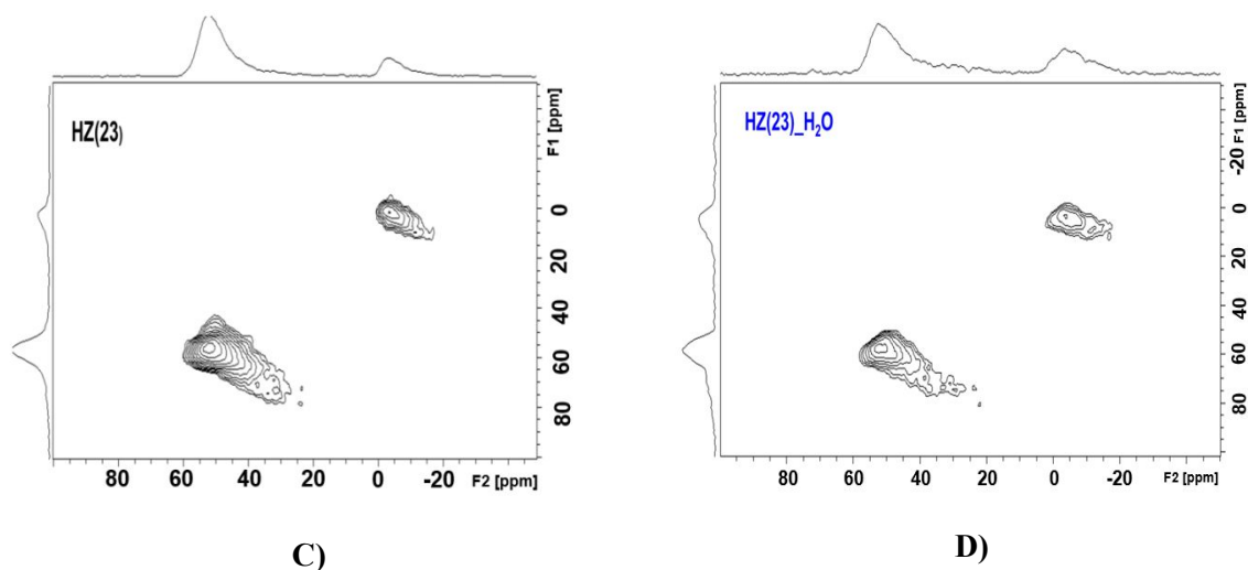
Figure 4. ^{27}\text{Al} MAS-NMR spectra of A) parent HZ(23) and water-treated HZ(23); B) HZ(80) and water-treated HZ(80). The C) and D) figures represent ^{27}\text{Al} 3QMAS-NMR data for HZ(23) and HZ(23) _{\text{H}_2\text{O}} respectively.
