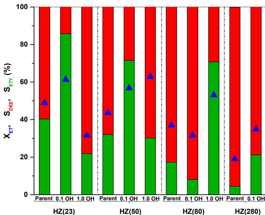
Figure 1. Conversion of ET (blue), selectivity of ETY (green) and of DEE (red) provided by parent HZSM-5 catalysts and by their counterparts treated in alkaline solution (values estimated at steady-state of reaction (5-6 h)). Test conditions: 225 °C, 1 bar, WHSV=35.7 h^{-1} .
