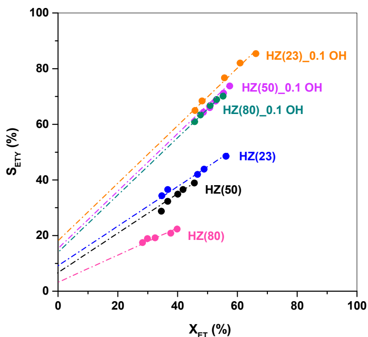
Figure 7. ETY selectivity ( S_{\text{ETY}} ) as a function of ET conversion ( X_{\text{ET}} , changed with WHSV) over HZ(23), HZ(50), HZ(80), HZ(23)_0.1 OH, HZ(50)_0.1 OH and HZ(80)_0.1 OH. Test conditions: 225 °C, total pressure \sim 1 bar, \text{WHSV}=17.9 - 89.1 \text{ h}^{-1} .
