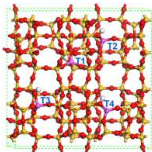
Fig. 9. The optimized periodic structure of HZSM-5 (atomic ratio Si/Al \sim 23, a = 20.615223 Å; b = 20.430119 Å and c = 13.716548 Å, \alpha = 90.0248 ; \beta = 89.76483 ; \gamma = 90.05055 .) Yellow: Si; Red: O; Purple: Al; White: proton.
