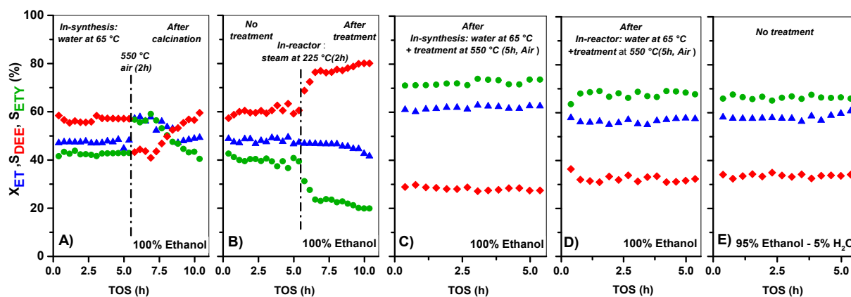
Figure 6. Evolution of ET conversion ( X_{ET} ), and selectivity to ETY ( S_{ETY} ) and DEE ( S_{DEE} ) as a function of TOS for: A) HZ(23) treated with water at 65 °C and in-situ calcined; B) HZ(23) treated in-situ with steam at 225 °C; C) HZ(23) treated with water at 65 °C and calcined ex-situ ; D): HZ(23) treated with water at 65 °C and calcined in-reactor; E) HZ(23) (only in H + -form) catalytic activity using 95%/5% ethanol/water as feed. All data shown for 225 °C, 1 bar total pressure and WHSV=35,7 h^{-1} .
