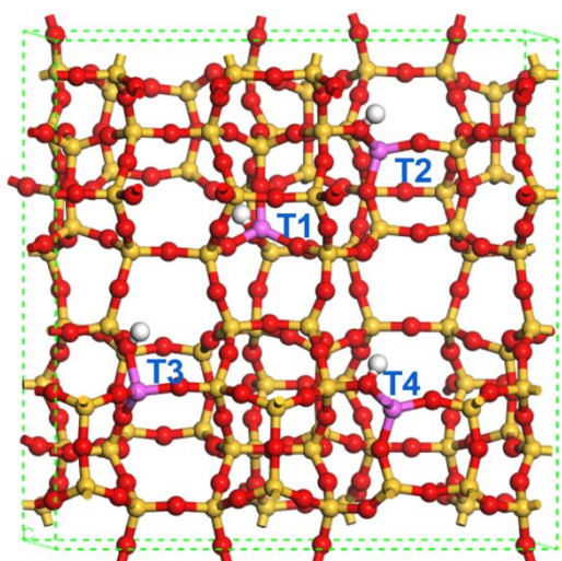
Fig. 9. The optimized periodic structure of HZSM-5 (atomic ratio Si/Al \sim 23 , a = 20.615223 \text{ \AA} ; b = 20.430119 \text{ \AA} and c = 13.716548 \text{ \AA} , \alpha = 90.0248 ; \beta = 89.76483 ; \gamma = 90.05055 .) Yellow: Si; Red: O; Purple: Al; White: proton.
