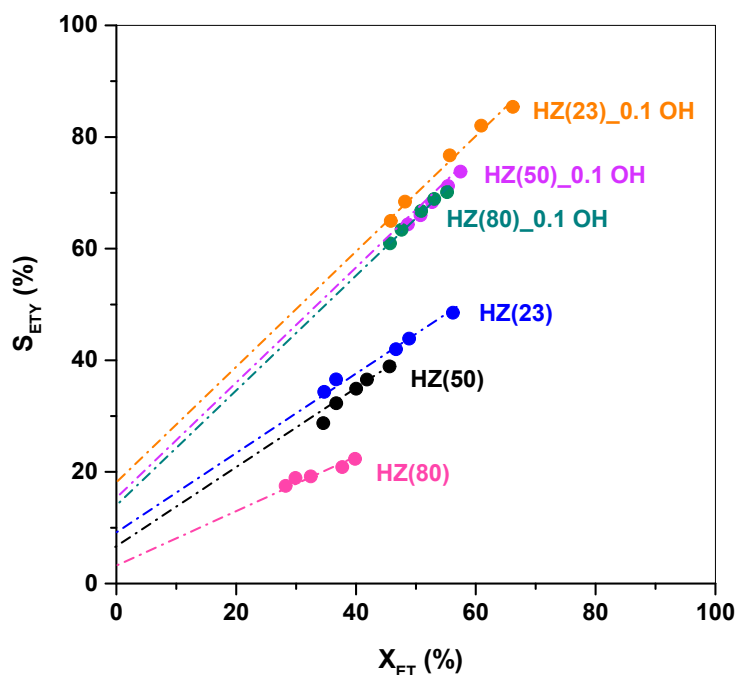
Figure 7. ETY selectivity ( S_{ETY} ) as a function of ET conversion ( X_{ET} , changed with WHSV ) over HZ(23), HZ(50), HZ(80), HZ(23)_0.1 OH, HZ(50)_0.1 OH and HZ(80)_0.1 OH. Test conditions: 225 °C, total pressure \sim 1 bar, WHSV=17.9 - 89.1 h^{-1} .
