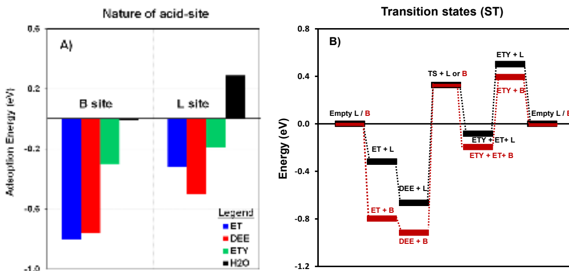
Fig. 10. A) The calculated adsorption energy (eV, Eq. 7) for ET, DEE, ETY and H 2 O on B site and L site for T2 position (-Al-); and B) Reaction coordinate diagram with DFT-derived energies normalized with respect to empty B or L sites at T2 positions. The TS for ET \rightarrow DEE is not shown for simplicity.
