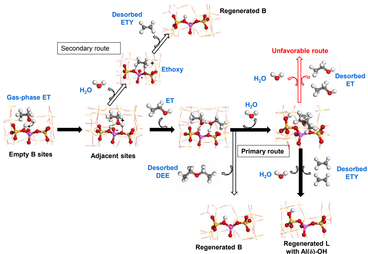
Scheme 1. Identified routes for ET-to-ETY over HZSM-5 at low-temperature reaction via: i) ET dimerization on neighboring sites on B species followed by DEE cracking on L ( primary route ), and ii) direct elimination of hydroxyl group of ET on B ( secondary route ).
