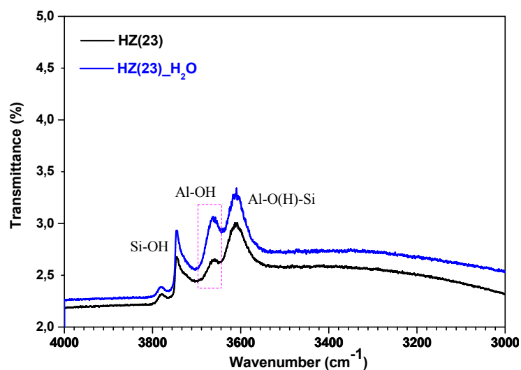
Figure 5. Normalized FTIR spectra on the OH-region for fresh parent HZ(23) and HZ(23) _{\text{H}_2\text{O}} samples evacuated in-situ at 350 °C (overnight) after ex-situ calcination at 500 °C (5h).
