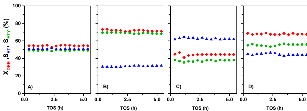
Fig. 8. Conversion of pure DEE ( X_{\text{DEE}} , red) and selectivity of ethylene ( S_{\text{ETY}} , green) and of ethanol ( S_{\text{ET}} , blue) as a function of TOS for: A) HZ(23), B) HZ(23)_0.1OH, C) HZ(80), and D) HZ(80)_1.0OH catalysts. Test conditions: 225 °C, 1 bar and \text{WHSV}=35.7 \text{ h}^{-1} .
