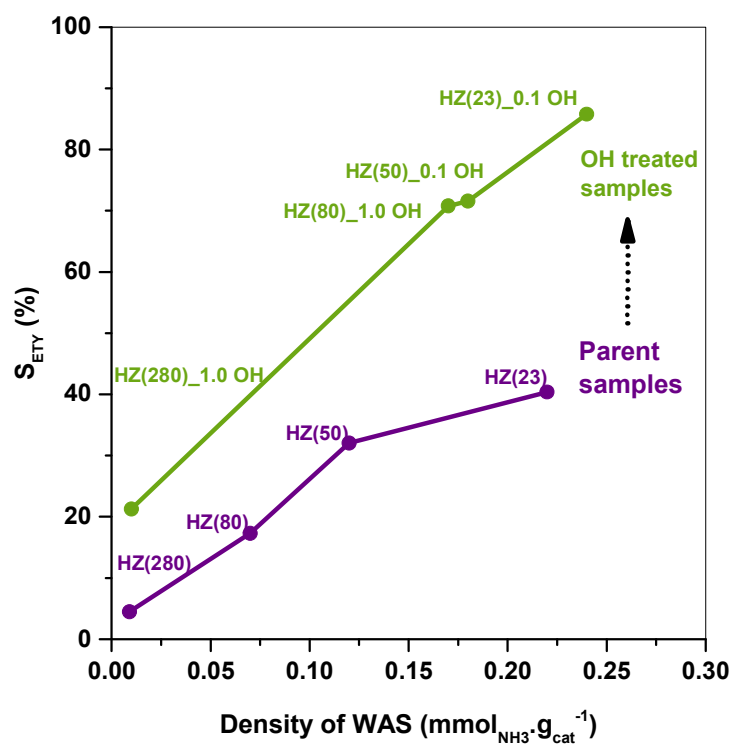
Figure 2. Correlation between the ETY selectivity (at similar ET conversion) and the density of WAS for parent (purple) and OH-treated (green) HZSM-5 catalysts tested at 225 °C, 1 bar, WHSV= 35.7 h^{-1} . S_{ETY} data are obtained under stable catalytic behaviors.
