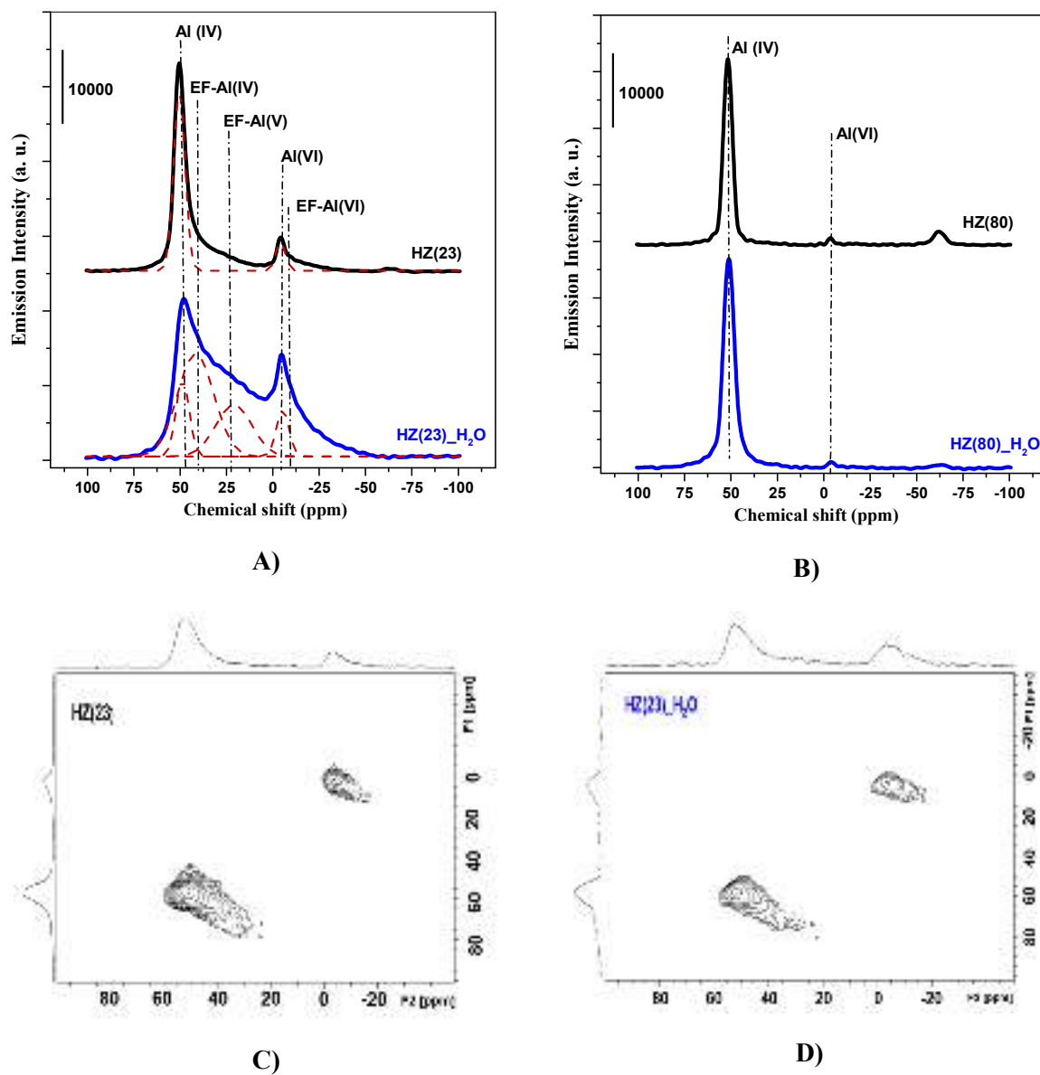
Figure 4. ^{27}\text{Al} MAS-NMR spectra of A) parent HZ(23) and water-treated HZ(23); B) HZ(80) and water-treated HZ(80). The C) and D) figures represent ^{27}\text{Al} 3QMAS-NMR data for HZ(23) and HZ(23)_H 2 O respectively.
