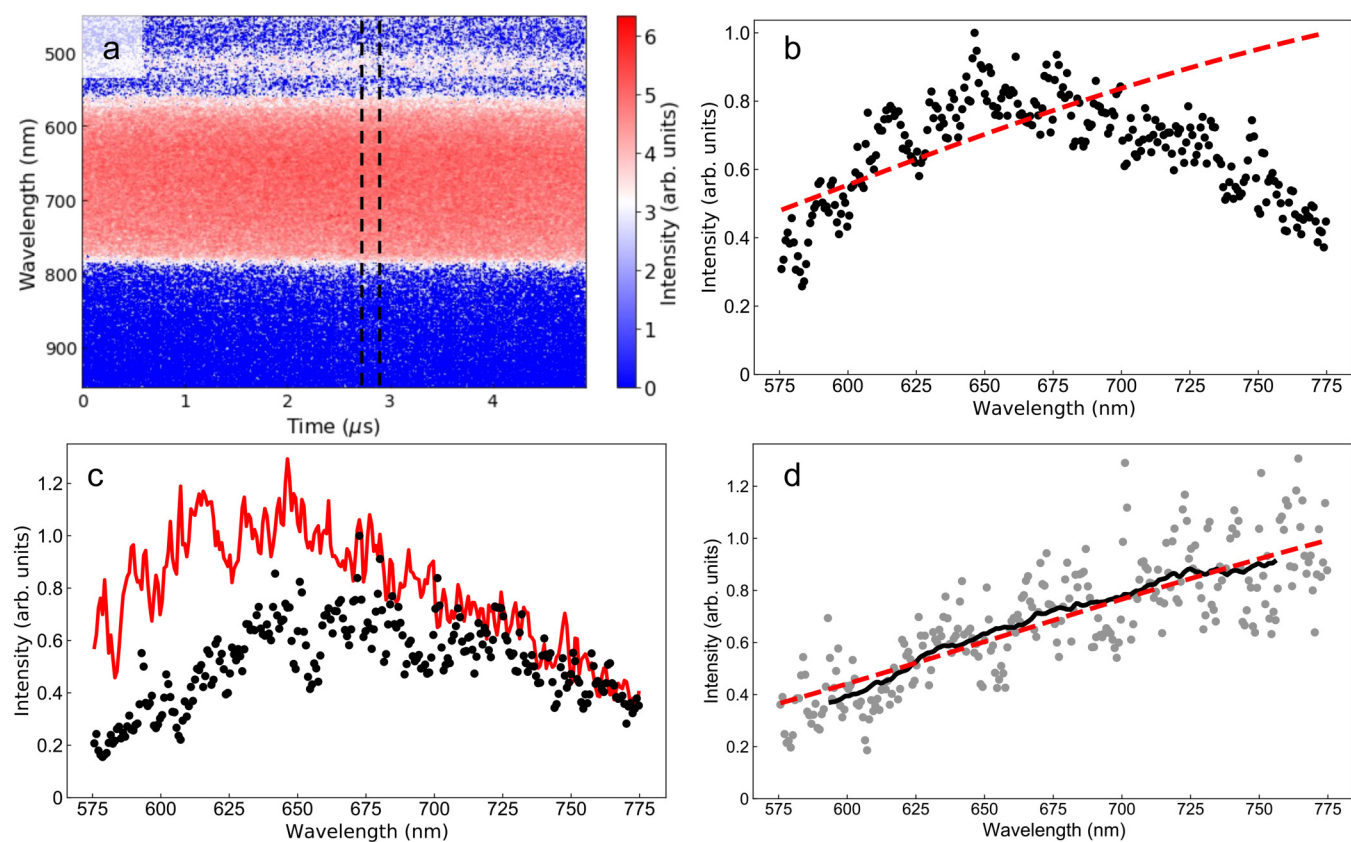
FIG. 6. Optical emission collected from the calibration lamp at 2500 and 2900 K. (a) Spectrogram of optical emission collected from a calibration lamp at 2900 K using a 5\ \mu\text{s} streak window, taken using enclosing trigger with a sweep repetition rate of 1 kHz and exposure time of 1 s. Region corresponding to 193 ns section binned at 2.8\ \mu\text{s} is shown between two dashed lines. (b) Binned optical emission at time = 2.8\ \mu\text{s} of calibration lamp at 2900 K (black markers) and expected optical emission of thermal radiation at 2900 K based on Planck's distribution (red dashed line). (c) Binned optical emission at time = 2.8\ \mu\text{s} of calibration lamp at 2500 K, black markers, and transmission function of full optical path at the same time (red solid line) derived from (b). (d) Corrected optical emission of calibration lamp at 2500 K, gray markers, at time = 2.8\ \mu\text{s} , with moving average intensity with respect to wavelength shown as a solid black line. The fitted Planck distribution (red dashed) to the corrected emission data at T = 2591 \pm 50\ \text{K} is also plotted.
