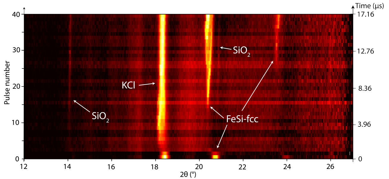
FIG. 3. Batch view of pulse train diffraction spectra series 23 . The pulse frequency was 2.25 MHz (time range span of 17.16 \mu s for 40 pulses). The moments where phases are first observed (spawn times) can be constrained by seeking the line apparition and checking for spots on the image plate. Observable phases are highlighted and designated. The KCl peak partly fades over the first pulses where the maximum fiber laser intensity is delivered to the sample, meaning that it is likely almost entirely molten inside the X-ray sampling zone. The first sample phase to crystallize upon cooling is \text{SiO}_2 . It is observed for the first time on the diffraction spectra at 2.2 \mu s (time zero corresponding to the first X-ray pulse). The FeSi-fcc peaks entirely disappear within the first 3 pulses before re-appearing at 5.72 \mu s for the left peak. Note that the second and fainter higher angle peaks of FeSi-fcc and \text{SiO}_2 appear later in time, likely due to signal degradation at higher angles and large crystal size.
