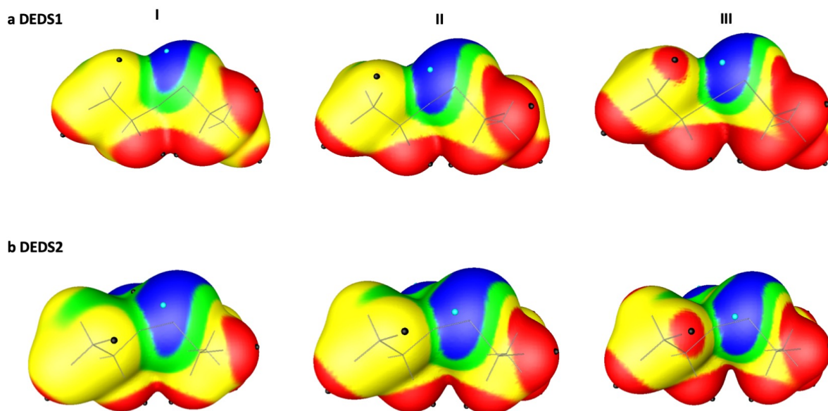
Figure 3: Separation of the electrostatic potential of the closest hydrogens plotted at the 0.001 a. u. (I) 0.002 a. u. (II) and 0.003 a. u. (III) iso-density surface for DEDES1 (a) and DEDES2 (b). The color ranges, in kcal/mol, are: red, greater 10; yellow, from 10 to 0; green, from 0 to -10; blue, more negative than -10.
