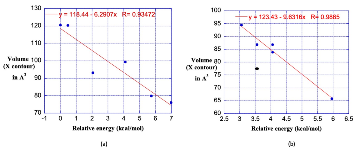
Figure 4. Plots of the nearly-touching contour X vs. relative energy of a conformer: a the DEDS series; b the PDB series (the data point for outlier PDB2 is shown, but was not included in the linear regression).
