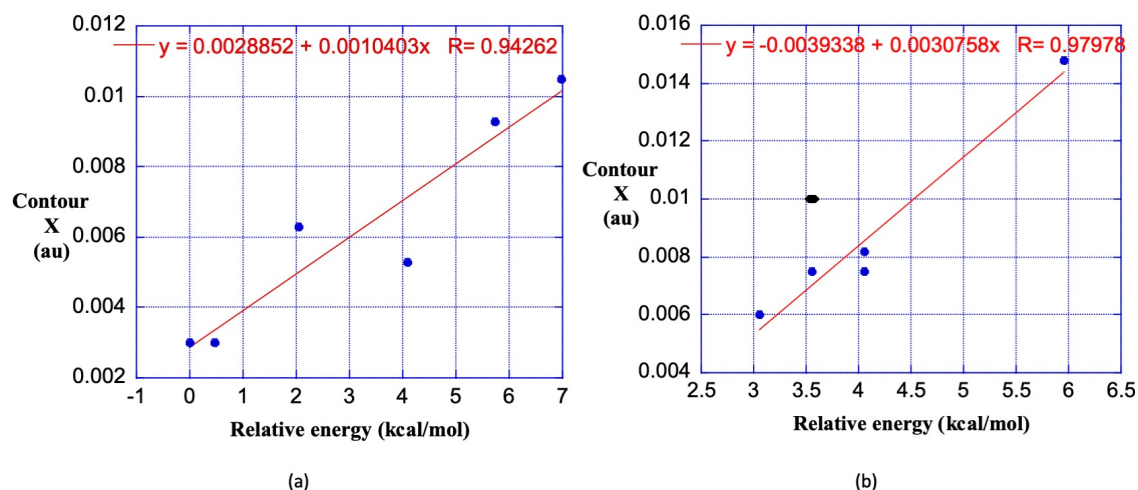
Figure 5. Plots of the nearly-touching contour X vs. relative energy of a conformer: a the DEDS series; b the PDB series (the data point for outlier PDB2 is shown, but was not included in the linear regression).
