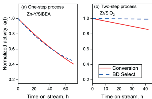
Fig. 14 Effect of time-on-stream on conversion and selectivity for catalysts in the one- and two-step processes. (a) ZnY/SiBEA ( T = 673 K, WHSV_{EtOH} = 1.0 h -1 ). 163 (b) Zr/SiO 2 ( T = 673 K, WHSV_{EtOH} = 1.5 h -1 ). 10
