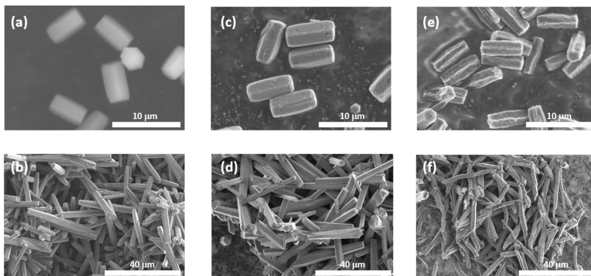
Fig. 4 SEM images of (a, b) 1 with different lengths obtained by the coordination modulation method, (c, d) 1 -PTh, and (e, f) PTh isolated from 1 . The morphologies and size of the recovered PTh objects retained those of the original hosts.
