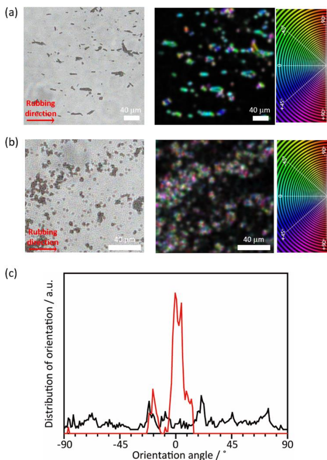
Fig. 6 (a,b) Microscope images and orientation analyses of (a) long and (b) short PTh rod particles after mechanical rubbing treatment. Orientation analyses were color-coded according to the orientation color map from -90^\circ to +90^\circ . (c) Angle orientation of the PTh rods with long (red) and short (black) length.
