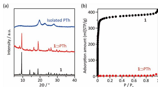
Fig. 3 (a) XRPD patterns of 1 , 1 \supset PTh, and PTh liberated from 1 . (b) \text{N}_2 adsorption isotherms of 1 and 1 \supset PTh at 77 K ( 1 ; S_{\text{BET}} = 1447 \text{ m}^2/\text{g} , 1 \supset PTh; S_{\text{BET}} = 4 \text{ m}^2/\text{g} ).
