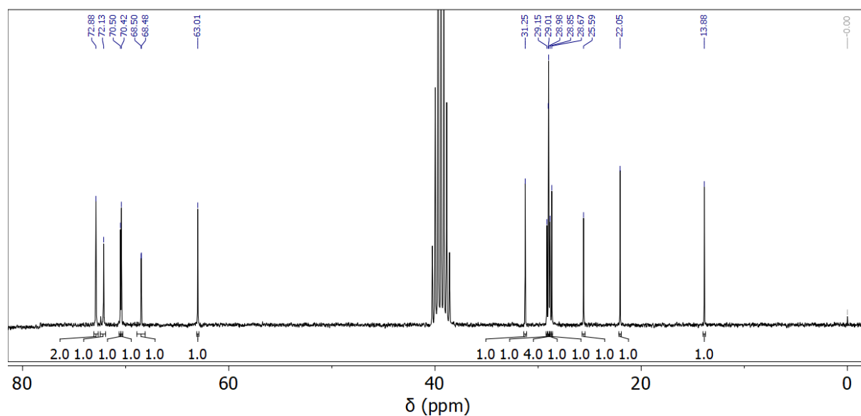
Figure S2. ^{13}\text{C} NMR (75 MHz) spectrum of 1-O-dodecyl diglyceryl ether in \text{d}_6 -DMSO. Peaks around 40 ppm corresponds to the solvent peak.
