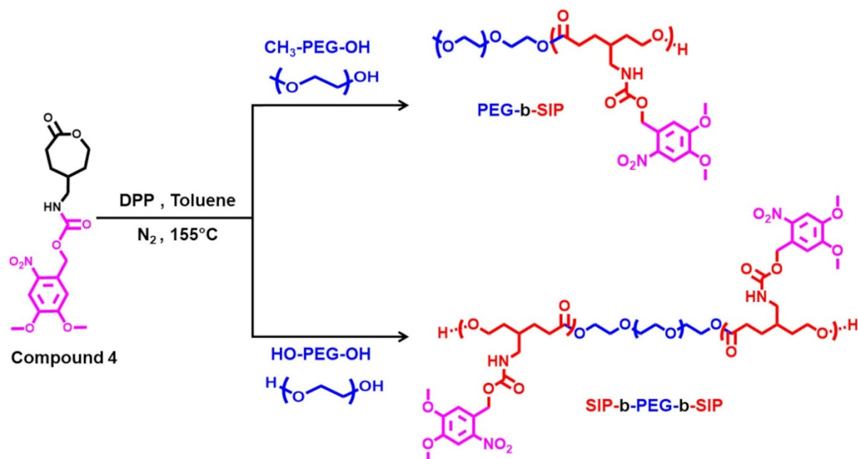
Scheme 1. Schemes of the synthesis of the diblock and triblock copolymers by ROP of Compound 4.
