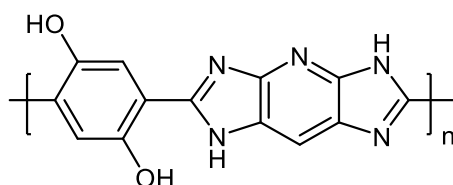
Figure 33. Repeat unit of Polypyridobisimidazole PIPD (M5)
