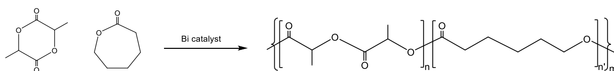
Scheme 4. Statistical LA-co-CL copolymer obtained with Bi[N(SiMe 3 ) 2 ] 3 catalyst
