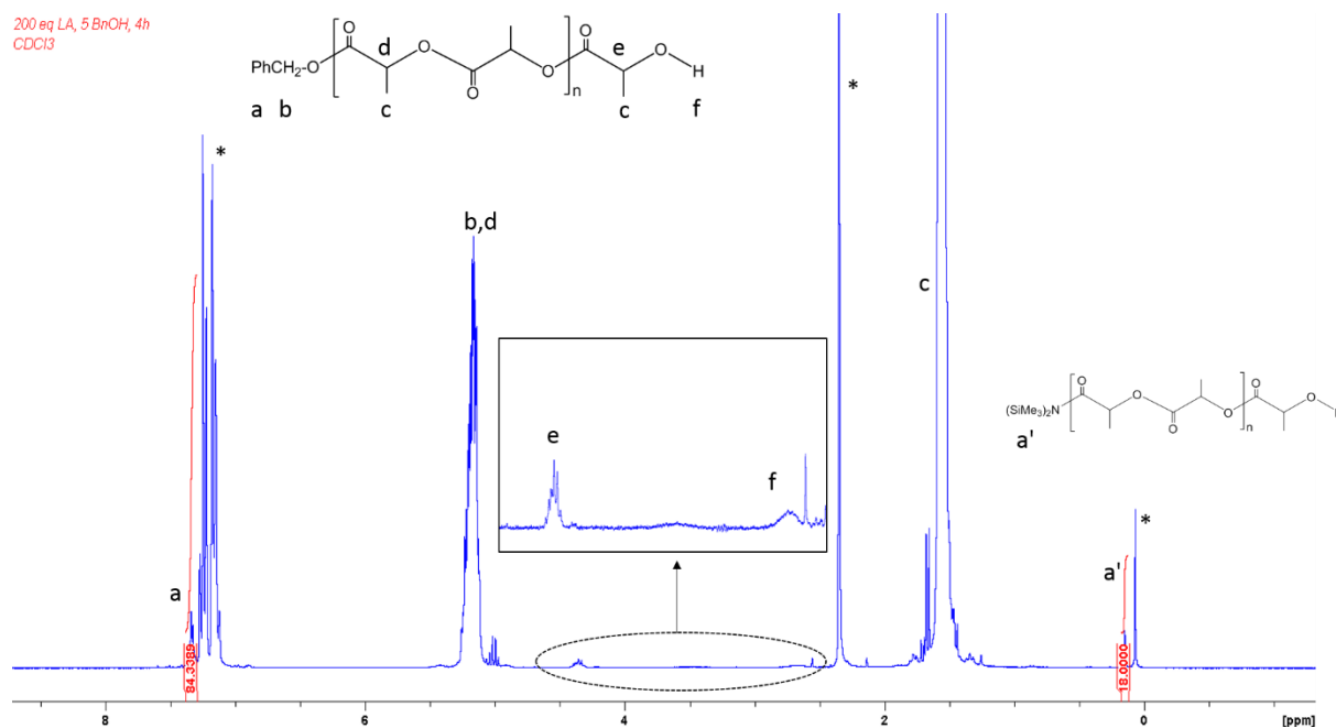
Fig. 1. 1 H NMR spectrum of PLA issued from run 8 for the determination of the chain end (in CDCl 3 , * toluene and silicone grease residues).
