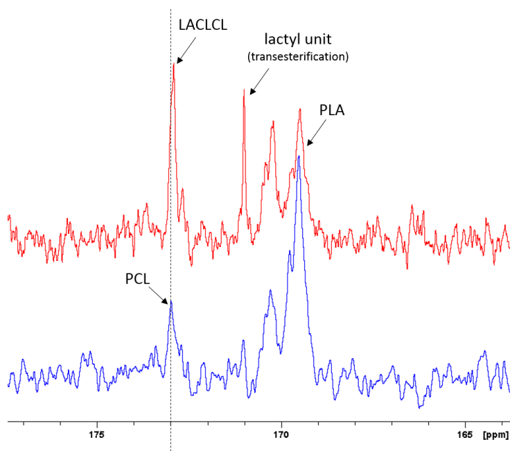
Fig. 3. ^{13}\text{C} \{^1\text{H}\} NMR region of copolymers issued from run 16 (bottom, blue) and run 17 (top, red) showing the increase of transesterification ( \text{CDCl}_3 ).
