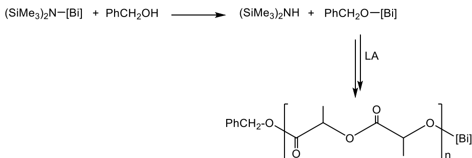
Scheme 2. Alcoholysis by BnOH prior to initiation (for one Bi-N bond) affording benzyloxy-terminated PLA chains.
