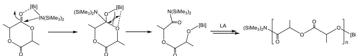
Scheme 1. Coordination-insertion mechanism affording amido-terminated PLA chains.
