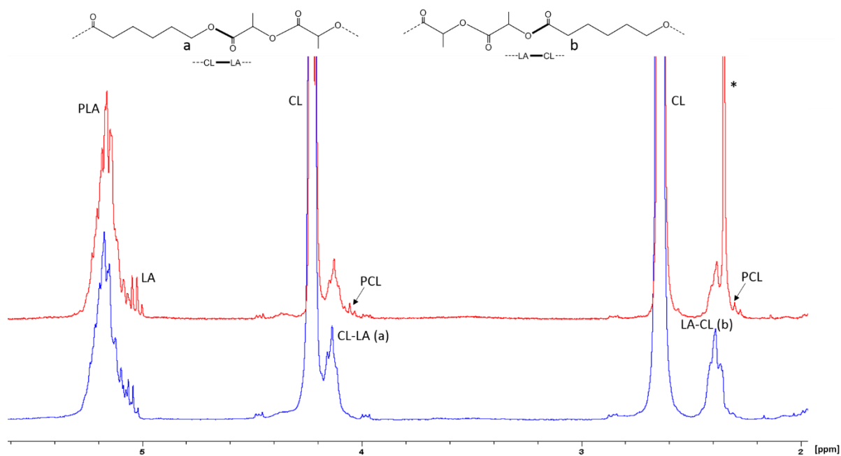
Fig. 2. ^1\text{H} NMR spectrum of the reaction mixture issued from run 14 (top, red) and run 16 (down, blue) showing the signals of the junction motives in the copolymer along with those of LA, CL, PLA, PCL ( \text{CDCl}_3 ).
