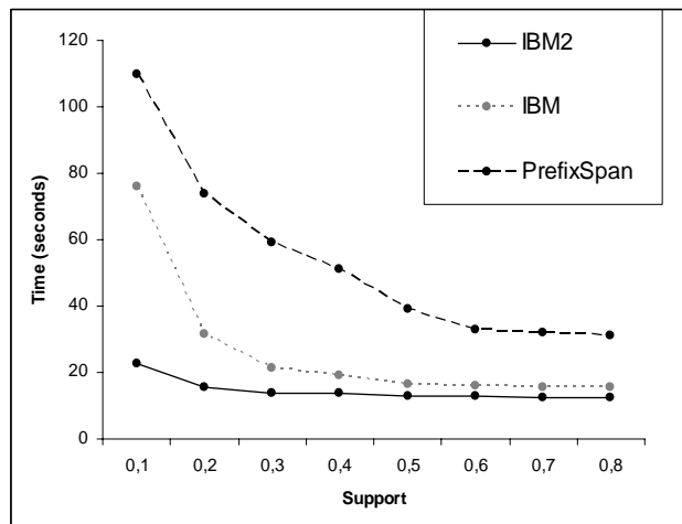
Figure 9. Performances with 600,000 rows
