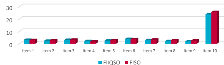
Figure 3 – CGVI scores
