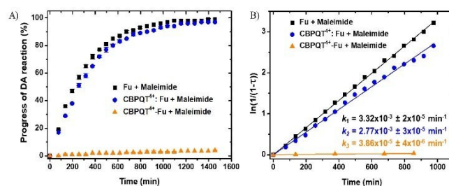
Figure 4. A) Diels-Alder reaction kinetics at 25 °C in water between maleimide (16 equiv.) and Fu (■), CBPQT 4+ :Fu (●) or CBPQT 4+ -Fu (▲), B) Plots of the ln(1/(1- \tau )) vs time in the DA reaction of maleimide with Fu (■), CBPQT 4+ :Fu (●), or CBPQT 4+ -Fu (▲). \tau is the conversion for the formation of cycloadducts. The pseudo-first-order rate constants ( k 1 , k 2 , k 3 ) were obtained from the slopes of the pseudo-first kinetic plots.
