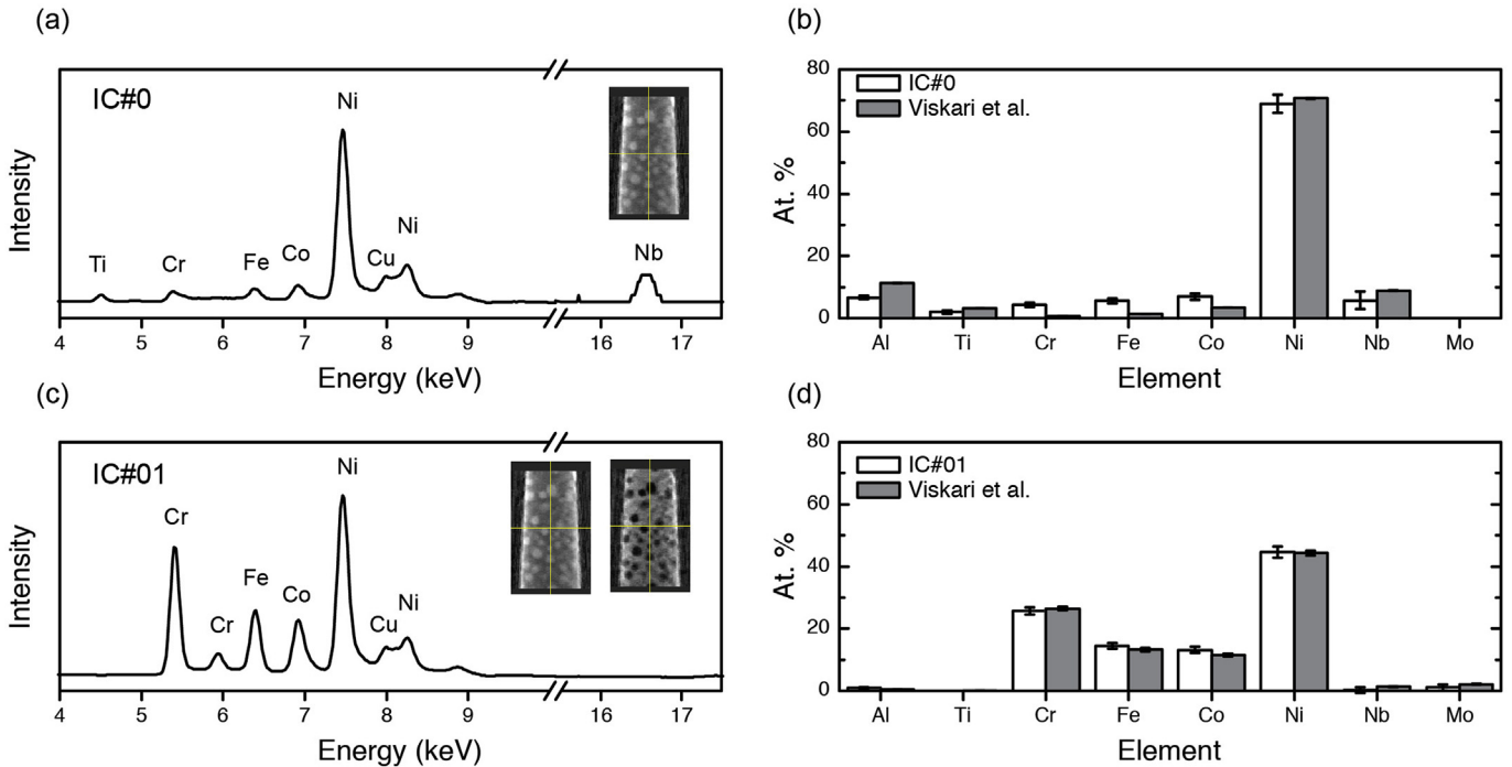
Fig. 7. A comparison of the composition of components IC#0 (a,b) and IC#01 (c,d) to APT determined compositions of the \gamma' and \gamma phases in 718Plus.
