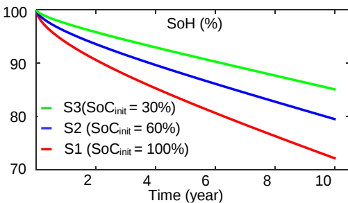
Fig. 15 SoH evolution for everyday charges
