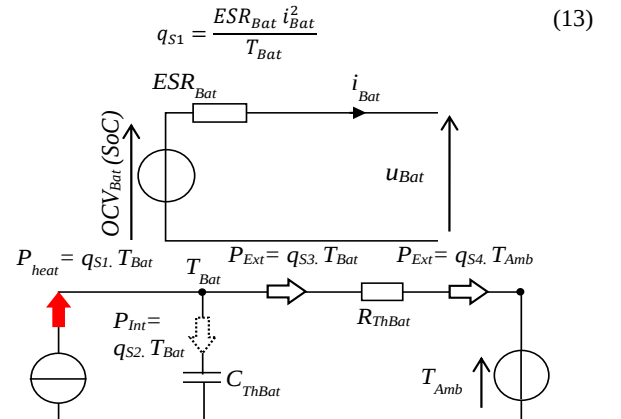
Fig. 8 Structure of the simplified electro-thermal model
