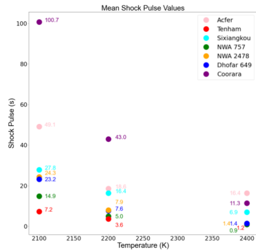
Figure 3 : Shock timescales obtained for an array of meteorites – two separate groups are clearly visible.
