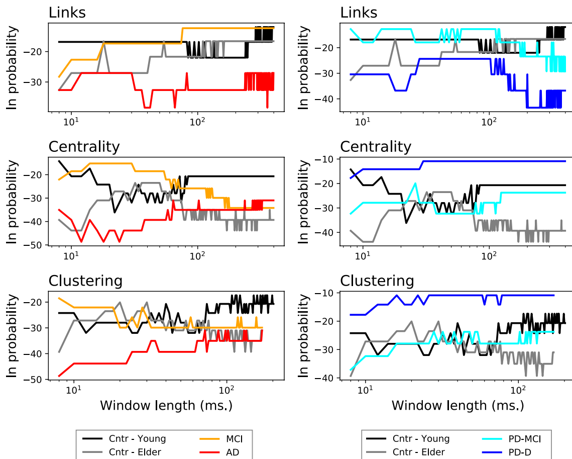
Figure 4. Intra-group stability. Evolution of the logarithm of the probability of finding the most frequent link with highest weight (top panels), and of the most frequent node with highest centrality (central panels) and highest clustering coefficient (bottom panels), as a function of the length of the window used to reconstruct the networks. Colour code of groups as in previous figures.
