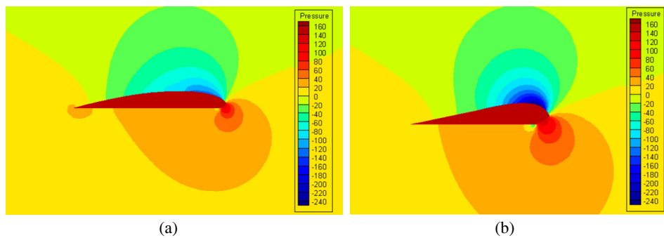
Figure 12. Pressure contours along chordwise of (a) Model C and (b) Model D at \alpha = 6^\circ .
