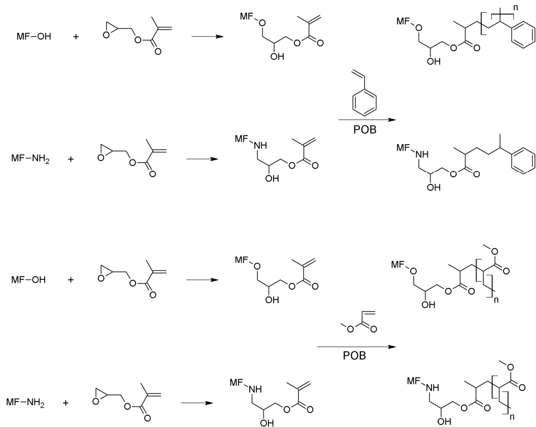
Figure 2. Proposed reaction between MF microcapsules, GMA, and styrene or methyl methacrylate.
