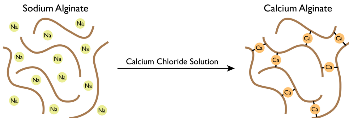
Figure 4. Gellification of sodium alginate solution.
