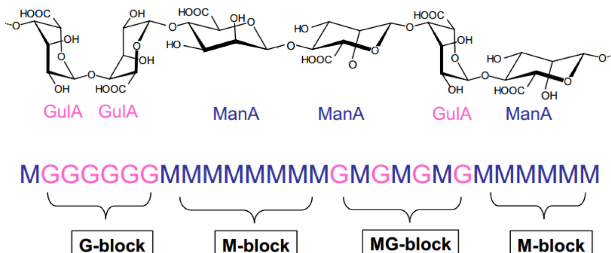
Figure 1. Alginate structure.
