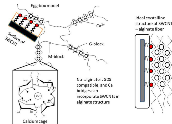
Figure 12. The interaction mechanism between CNT and alginate [96].
