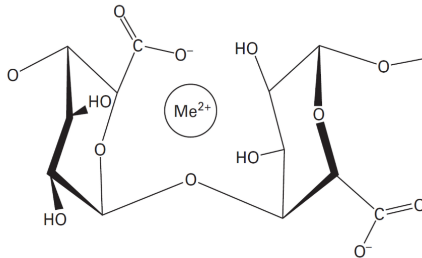
Figure 2. The stereo-chemical structure of the GG block [25].
