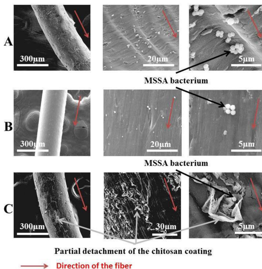
Figure 17. Scanning electron microscope observation of alginate fibers (A), chitosan fibers (B), and alginate-reinforced chitosan fibers (C) [126].
