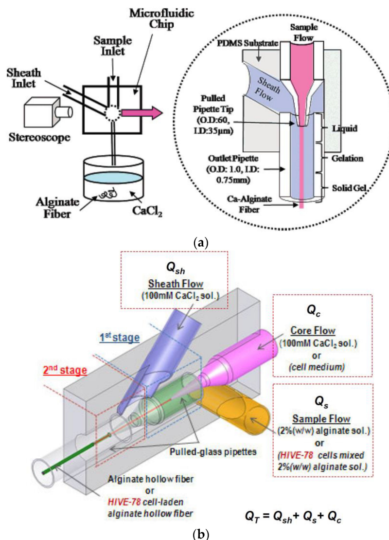
Figure 6. Microfluidic concept for (a) continuous alginate micro-fibers and (b) continuous alginate hollow micro-fibers.
