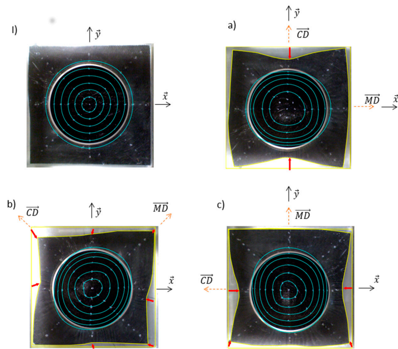
Figure 9. Initial state (I) and preformed nonwoven specimens at 0°, 45°, and 90° angles for nonwoven material MD-axis relative to the machine x-axis (a–c, respectively). Red bold arrows indicate the maximum draw-in.
