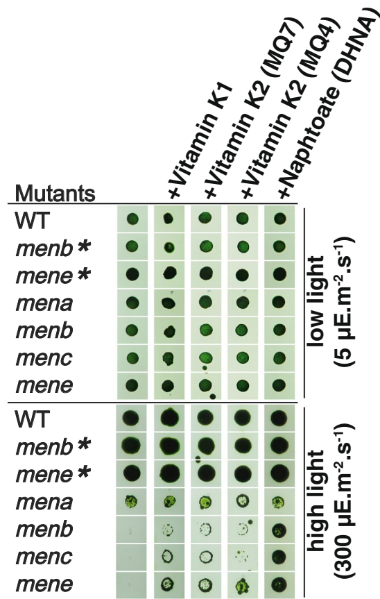
Figure 6. Growth of control and menaquinone mutant strains under different culture supplementation conditions. 20 \mu\text{l} of cell culture at 106 cells. \text{ml}^{-1} were spotted on classical TAP media, or supplemented media with either Vitamin K1, Vitamin K2 (MQ7), Vitamin K2 (MQ4), or Naphthoate (DHNA) and then submitted to either high or low light conditions for 7 days. The "*" indicate mutants rescued by supplementation.
