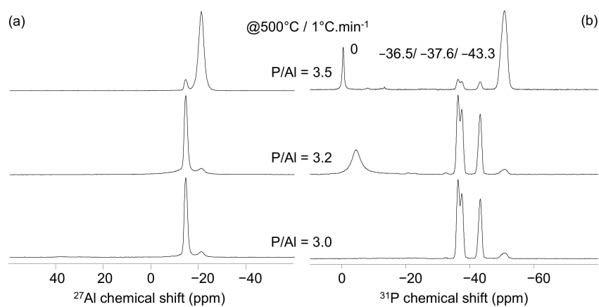
Figure 3. ^{27}\text{Al} (a) and ^{31}\text{P} (b) MAS-NMR spectra obtained at 500 °C on Al/P = 3 (bottom), 3.2 (middle), and 3.5 (top) solutions.
