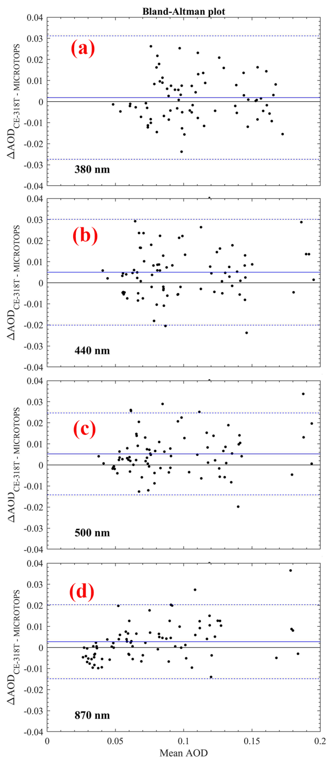
Figure 5. Bland–Altman plots for AOD differences with mean AOD ((AOD_{CE-318T} + AOD_{MICROTOPS})/2) at 380 (a), 440 (b), 500 (c) and 870 nm (d). The solid black-colored and blue-colored lines represent the zero line and the mean AOD differences, respectively. Dotted blue-colored lines represent the mean AOD plus/minus the root-mean-squared AOD differences.
