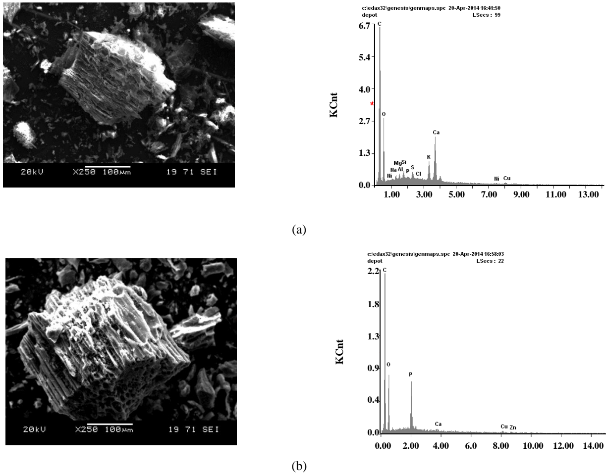
Fig. 1: SEM picture and EDX microanalysis of : (a) carbonized precursor and (b) activated plant.
