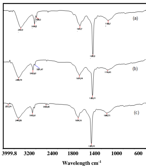
Fig. 2: FTIR spectra of AC (a), carbonized precursor (b), AC after sorption (c).
