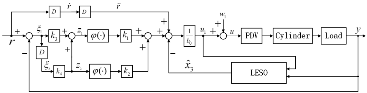
FIGURE 3. Block diagram of the closed-loop electro-hydraulic position control system regulated by the proposed controller.
