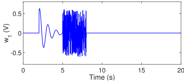
FIGURE 9. The external disturbance w_1 reduces from 0.6237 V to -0.3692 V during the time interval [2.06 s, 2.6 s]; w_1 varies randomly between -0.6 V and 0.6 V when 5 \leq t < 8 s.
