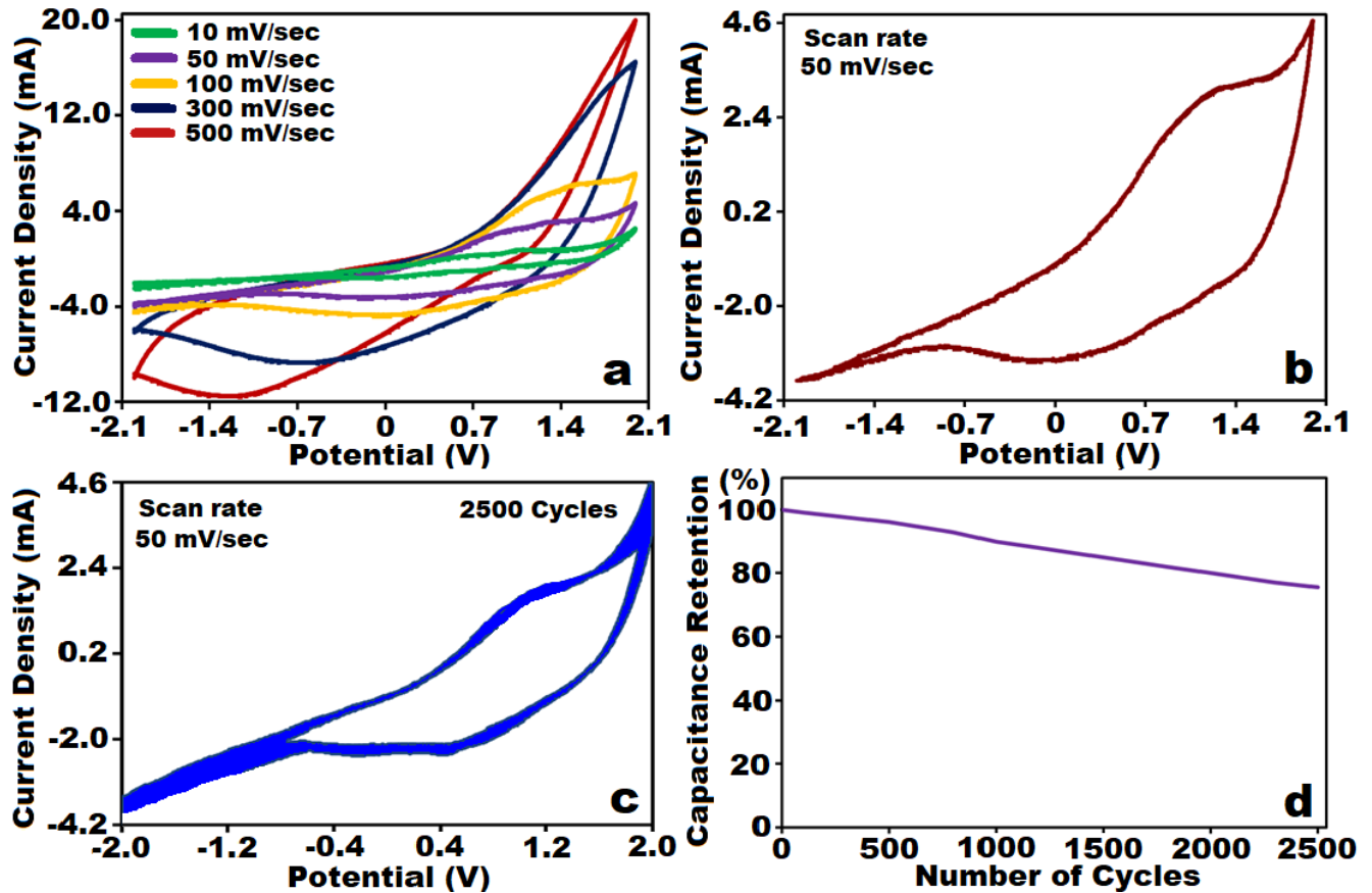
FIGURE 4. Electrochemical testing and life cycle analysis of the display device. (a) Cyclic Voltammetry (CV) operation of the electrochromic device in the range of -2.0 to +2.0 V with the scan rate of 10 mV/sec to 500 mV/sec. (b) CV analysis on 50 mV/sec scan rate for electrochromic device. (c) Stability analysis by performing 2500 cycles of CV analysis at 50 mV/sec scan rate. (d) Stability investigation by plotting the specific capacitance retention percentage over the number of cycles.
