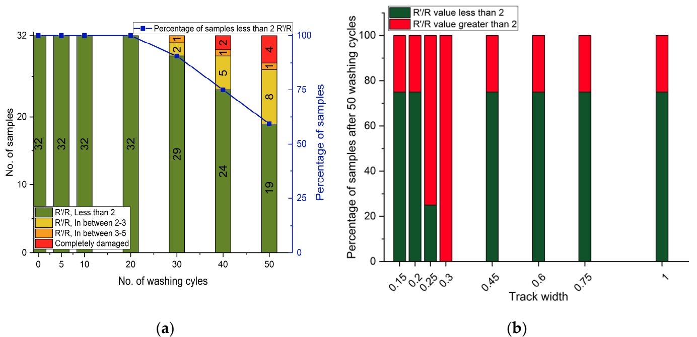
Figure 6. FPCB sample (with silicone protection completely) analyses after 50 Express washing cycles, a total of 32 samples were tested: (a) No. of samples with R'/R values increased above 2, 3, and ultimately damaged pieces on the left y-axis and percentage of samples having R'/R value below 2 on the right y-axis; (b) ratio of samples having R'/R values below and above 2 after complete washing cycles based on track widths.
