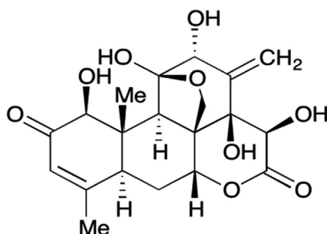
Figure 1: Eurycomanone structure
