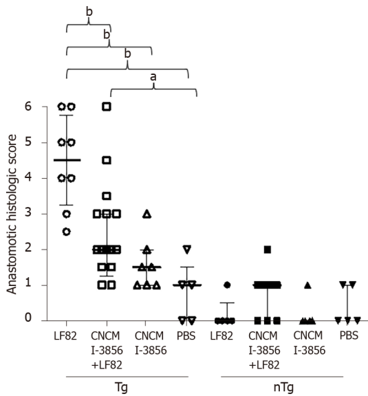
Figure 5 Anastomatic histologic lesions at sacrifice. Anastomatic histologic scores in the different groups of HLA-B27 transgenic (Tg) rats and wild-type (nTg) rats at sacrifice. a P < 0.05, b P < 0.01. LF82: Adherent-invasive Escherichia coli strain LF82; CNCM I-3856: Saccharomyces cerevisiae CNCM I-3856; PBS: Phosphate buffered saline.
