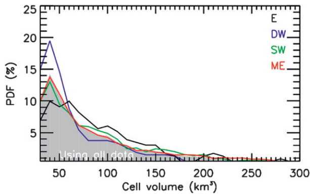
FIG. 7. As in Fig. 3a, but for the PDFs of TITAN cell volume using a bin size of 20 \text{ km}^3 .
