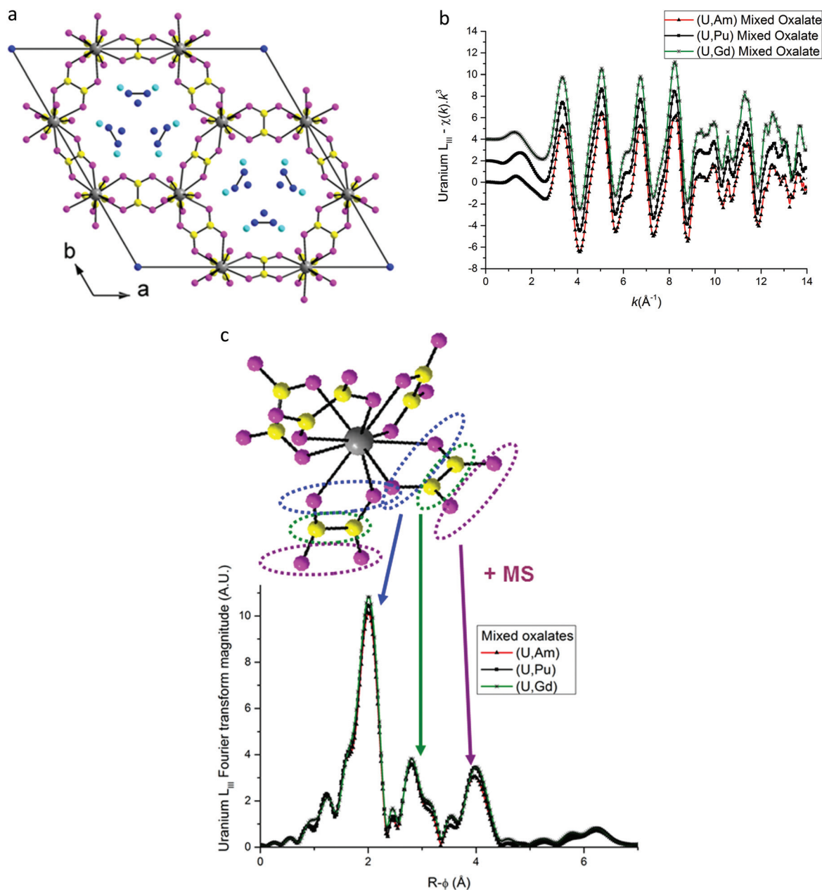
Fig. 6 (a) Hexagonal unit cell based on resolved (U,Nd) structure. 24 (●) Actinide/lanthanide cations, (●) and (●) oxygen and carbon atoms in the C 2 O 4 group, and (●) monovalent cations and (●) oxygen atoms in water molecules. (b) EXAFS data at uranium L III edge. (c) Fourier transformations of EXAFS shown in (b).
