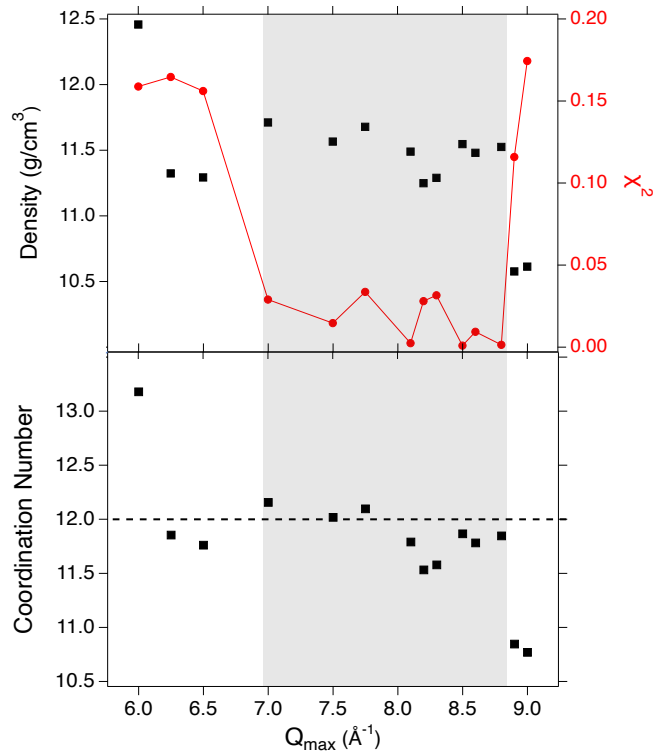
FIG. 8. Effect of Q_{\text{max}} on optimization - shot 831. Density and \chi^2 (top) and coordination number (bottom) was determined as a function of Q_{\text{max}} . The figure of merit \chi^2 (red) is minimized between 7.0\text{-}8.8 \text{\AA}^{-1} .
