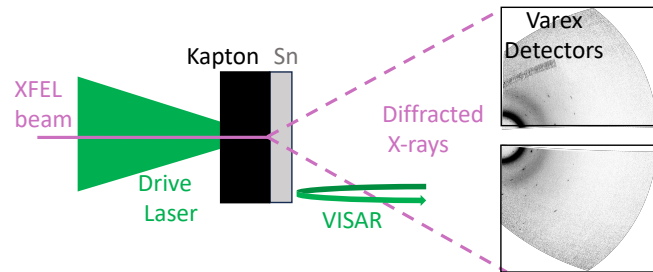
FIG. 1. Experimental setup. The target design consists of a 50 \mu\text{m} thick polyimide ablator bonded to a 20 \mu\text{m} thick Sn foil with a \sim 1 \mu\text{m} glue layer. Diffraction data from laser shock compressed Sn at an estimated pressure of 85(5) GPa is shown. The 2D diffraction images were generated using the HEXRD diffraction software package 13
