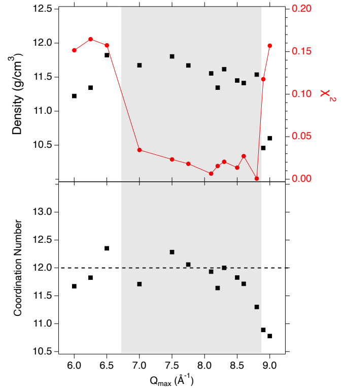
FIG. 6. Effect of Q_{max} on optimization - shot 826. Density and \chi^2 (top) and coordination number (bottom) as determined as a function of Q_{max} . The figure of merit \chi^2 (red) is minimized between 7.0 - 8.8 \text{ \AA}^{-1} .
