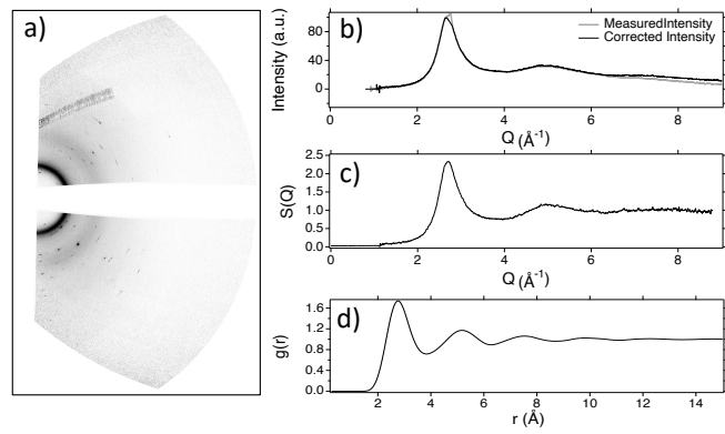
FIG. 7. Structural analysis of liquid Sn - shot 831 (a) 2D diffraction image warped into geometric view such that diffraction rings are concentric circles. (b) 1D integrated line out from uncorrected and corrected data. (c) Optimized S(Q) profile. (d) Optimized g(r) profile.
