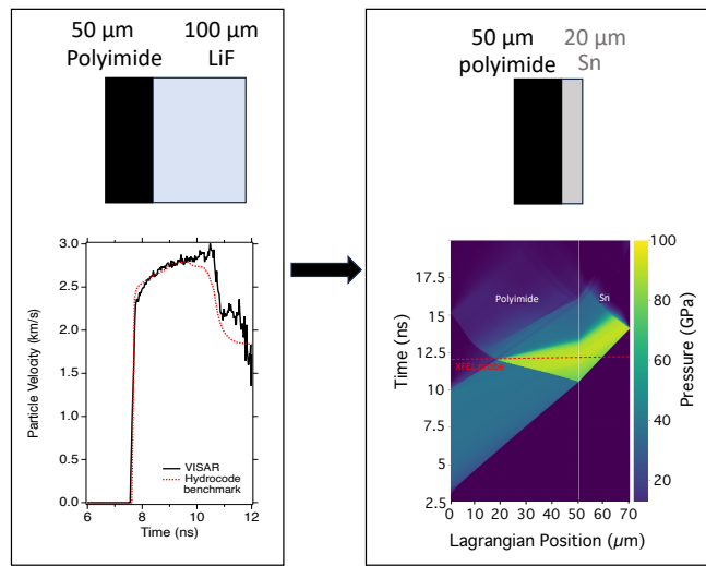
FIG. 2. Pressure Determination Experiments performed on polyimide - LiF targets are used to benchmark hydrodynamic simulations (left) which are then used to predict the pressure conditions reached in experiments which used polyimide-Sn targets at identical laser energies (right).
