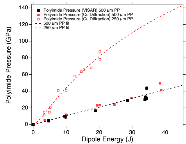
FIG. 3. Polyimide pressure as a function of laser energy for 500 \mu\text{m} and 250 \mu\text{m} phase plates (PP). This relation was determined by two independent methods: using impedance matching from VISAR traces from polyimide-LiF targets (black); using impedance matching from Cu diffraction data from polyimide-Cu targets (red).
