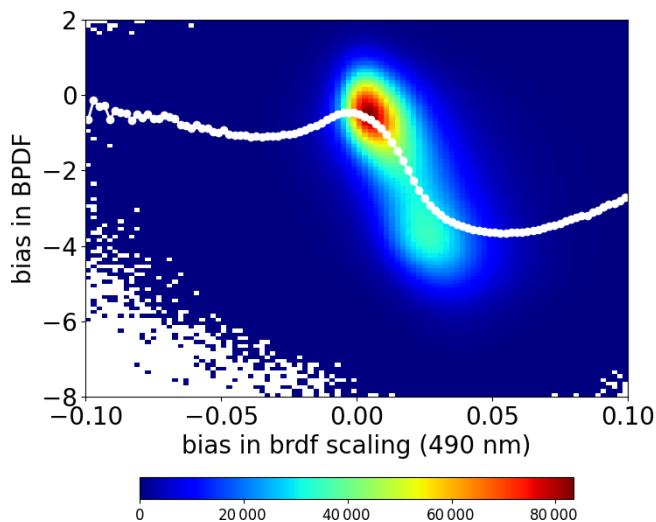
Figure 18. Difference in BPDF scaling parameters as a function of the difference in the isotropic BRDF parameter (490 nm). Differences represent RemoTAP–GRASP. The x axis and y axis have been divided into 100 bins. The white circles indicate the median y value per x bin. The color indicates the number of data points per bin.
