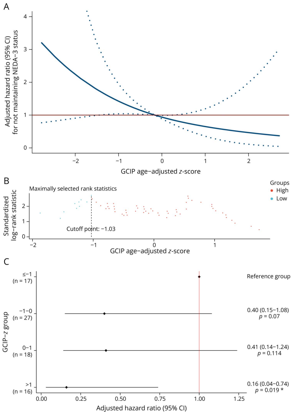
Figure 3 Association Between Risk of Future Disease Activity and GCIP z Scores in PwEMS
