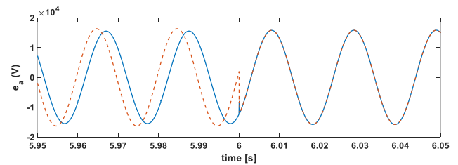
Fig. 10: Comparison of Phase A Voltage at BESS 2 level: Converter Side (red) and Grid Side (blue).
