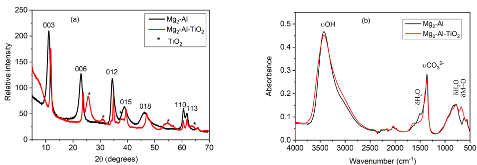
Fig. 2. (a) X-ray diffraction diagrams and (b) ATR-FTIR spectra of Mg 2 -Al and Mg 2 -Al-TiO 2
